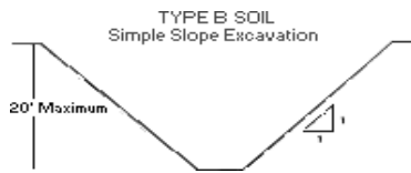
Figure 4 - Normal Sloping configuration for a “type B soil”.
